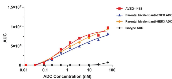
Figure 21 – AVZO-1418 internalization in EGFR/HER3 co-expressing cells.
