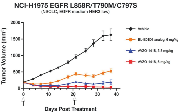
Figure 23 – AVZO-1418 in an osimertinib-resistant NSCLC model.
