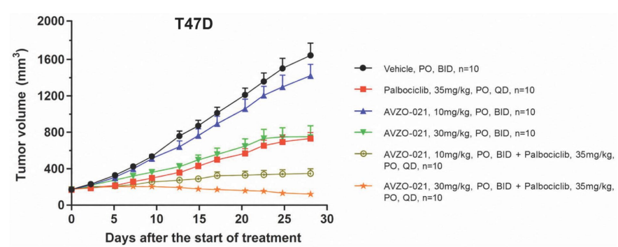
Figure 7 – AVZO-021 in combination with CDK4/6 inhibitors in the T47D xenograft model.
